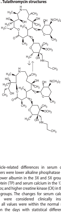
Figure 1. Tulathromycin structures
