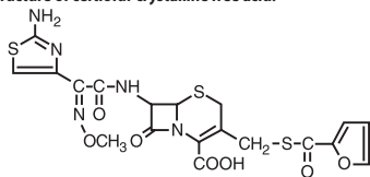
Figure 1. Structure of ceftiofur crystalline free acid:
